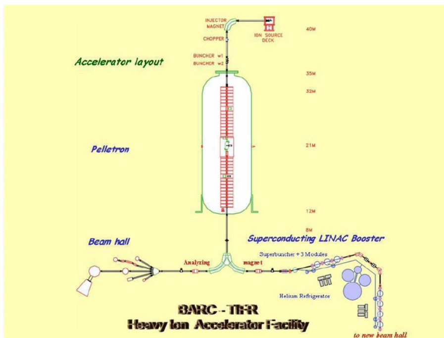
Fig. 4.1.2: Schematic showing the BARC-TIFR heavy ion accelerator facility.
