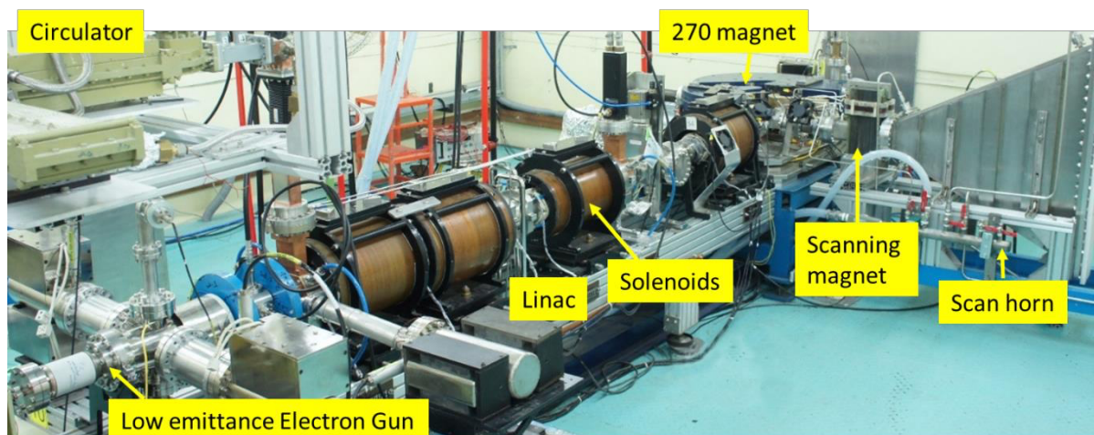
Fig. 4.7.1: Photograph of the 9.5 MeV, 10 kW industrial electron linac developed at RRCAT.
