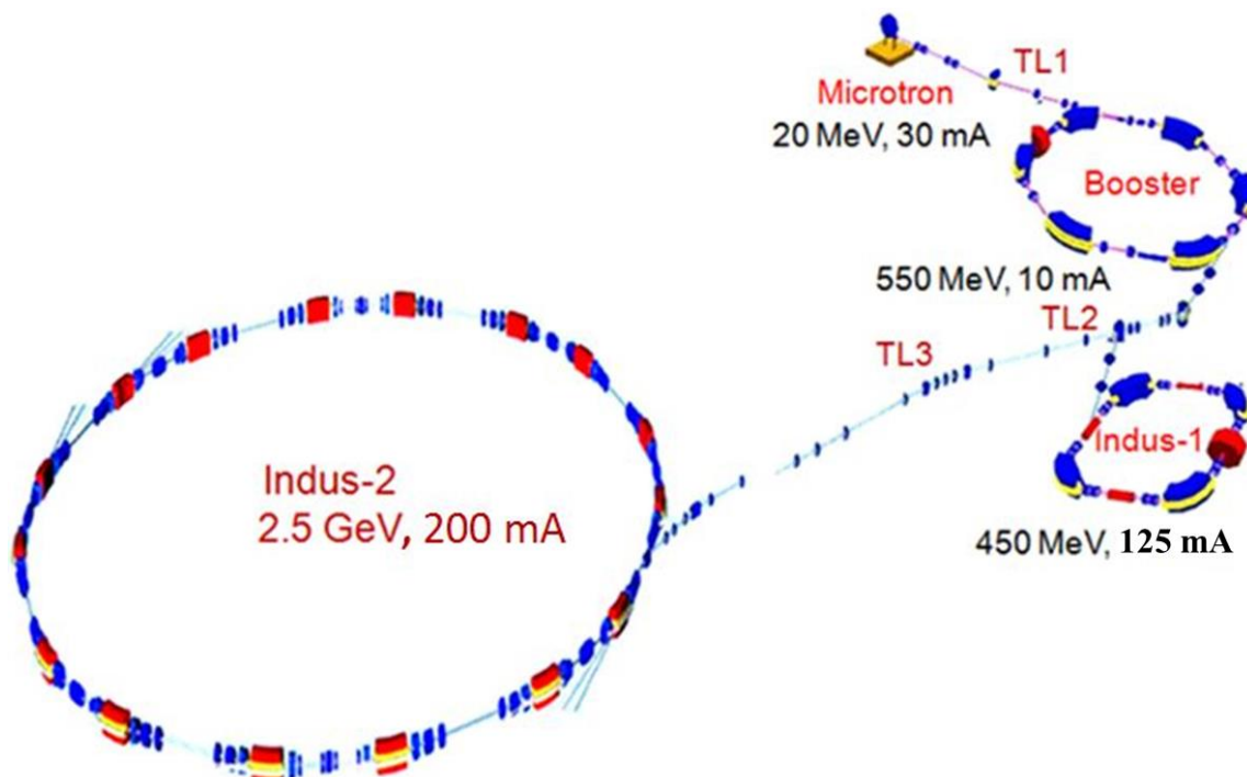
Fig. 4.2.1: Schematic showing different accelerators in Indus accelerator complex
