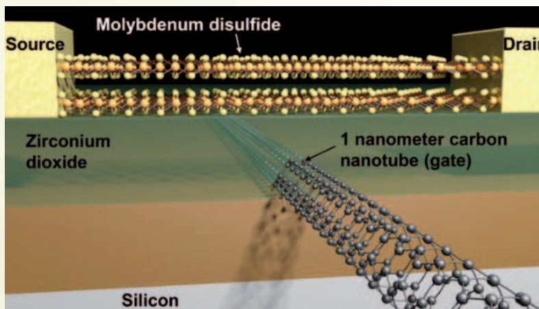
MoS 2 transistor with 1-nanometre carbon nanotube gate.
