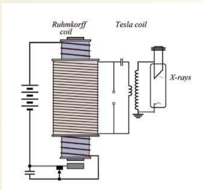
Fig.3. Schematic diagram of X-ray apparatus in which a Tesla coil coupled with Ruhmkorff coil used as a high-voltage source, as was possibly used by Jagadis Chandra Bose.
