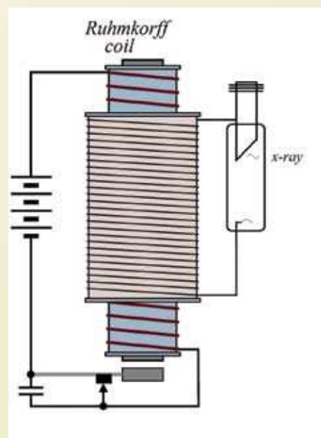
Fig.2. Schematic diagram of X-ray apparatus using a Ruhmkorff coil as a high-voltage source as was used by Roentgen.
