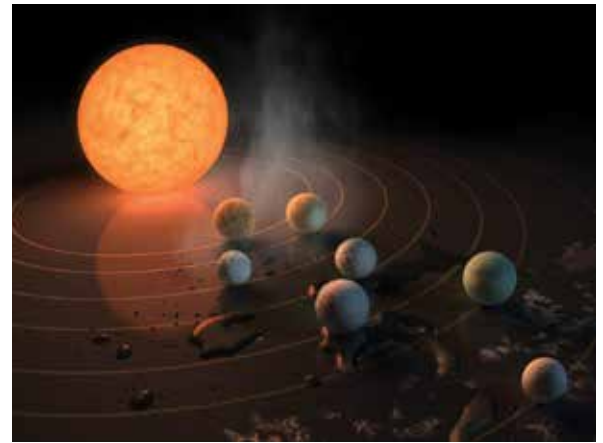
Fig. 1. An artist's impression of the seven planets orbiting a dwarf star (Credit: Nature)
