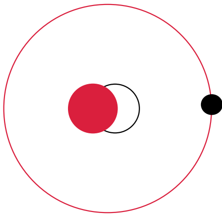
Fig.2. A star-planet system orbiting a common centre of mass
