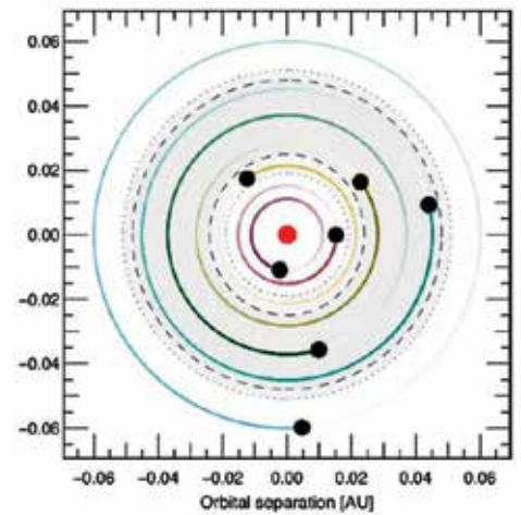
Fig.4. Orbits of seven planets around the cool star TRAPPIST 1a. The shaded areas and the dashed circles represent habitable zones around the star under various assumptions.
