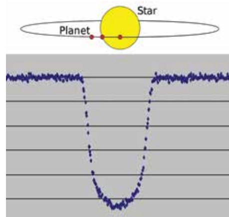
Fig.3. A planet transiting its star and the resulting dip the starlight as seen by observer on Earth. The dip is exaggerated (Credit: Wikipedia)
