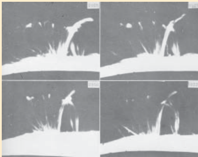
Fig. 4 : Prominence activity on the Sun, a spectacular loop prominence on the SE-limb (November 26, 1982), USAO
