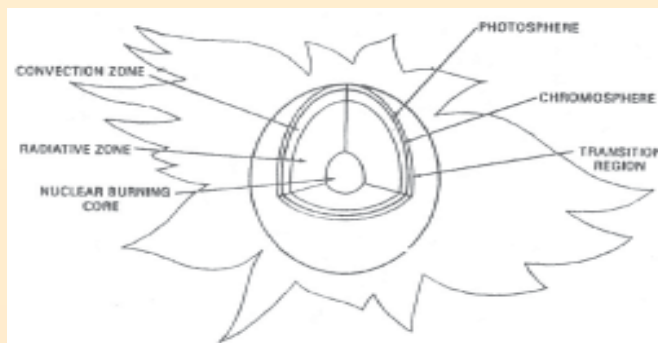
Fig. 2 : Inner layers of the Sun, with the solar corona in the background
