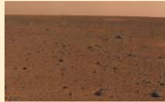
Martian surface
