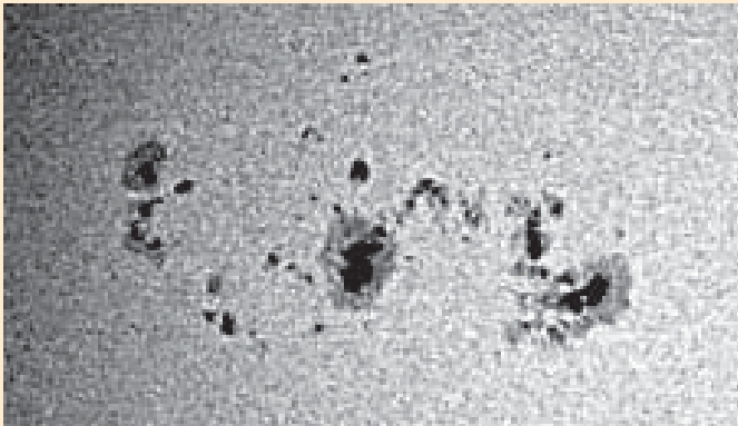
Fig. 3 (A) : Sunspots on the surface of the Sun. The lower figure is the magnified view of the sunspots observed in the upper one
