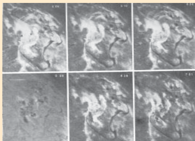
Fig. 5 : Multi-ribbon flare observed on May 13, 1981 during 0505 UT to 0701 UT, USAO
