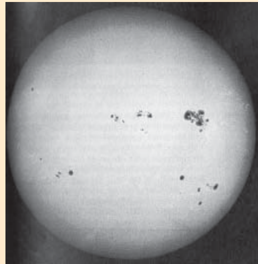
Fig. 3 (B) : Sunspots when the solar activity is high
