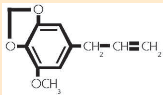
Figure 3: Molecular structure of Myristicin
